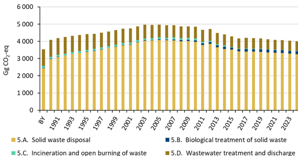
Figure 7.1.1 Trend of emissions of the different categories in waste sector
