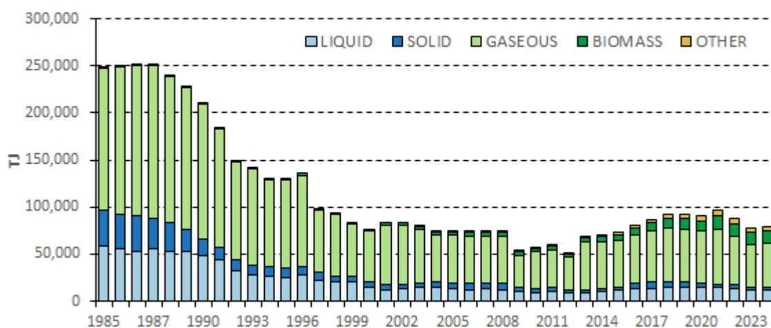
Figure 3.2.6.2 Fuel combustion in the Manufacturing Industries and Construction Sector (1990-2024)
