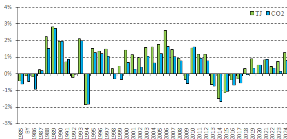
Figure 3.2.3 Differences between the reference and the sectoral approach as regards fuel consumption and CO 2 emissions
