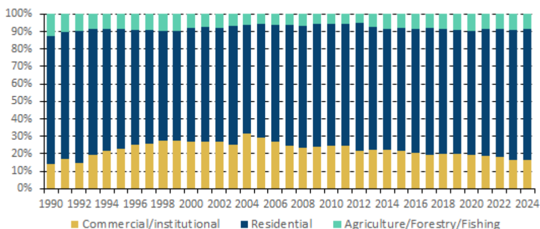
Figure 3.2.8.3 Fuel combustion in the subsectors of the Other Sector (1990-2024)
