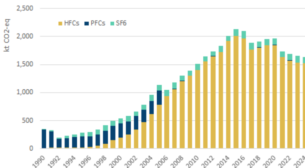
Figure 2.13 Trend of F-gas emissions (1990-2024)
