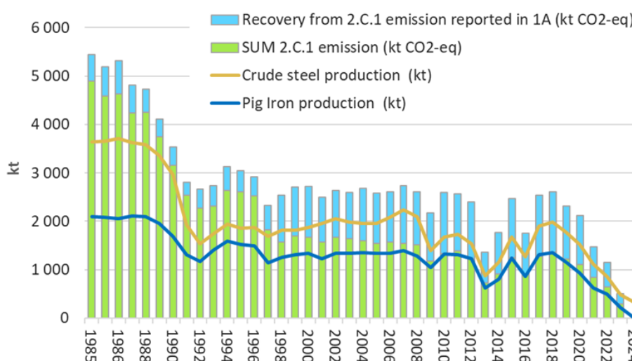
Figure 4.5.1 Trend of production and emissions in Iron and steel sector
