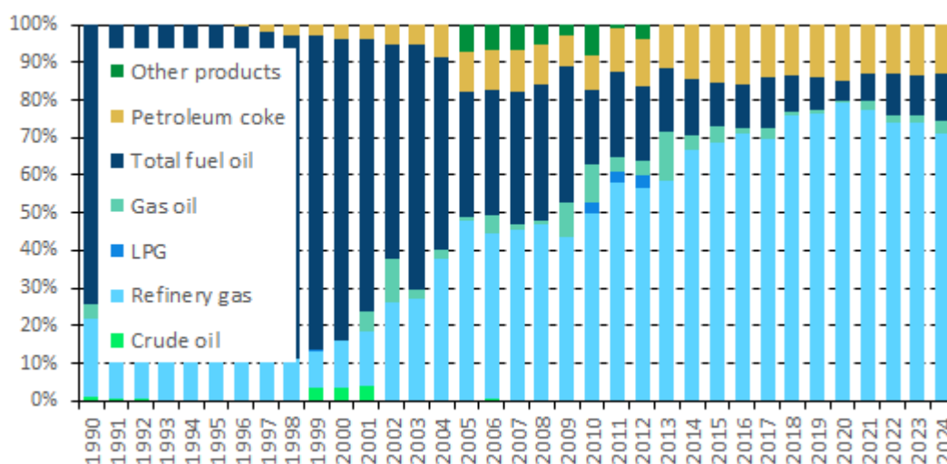
Figure 3.2.5.6 Share of different liquid fuels used by energy industries (1990-2024)
