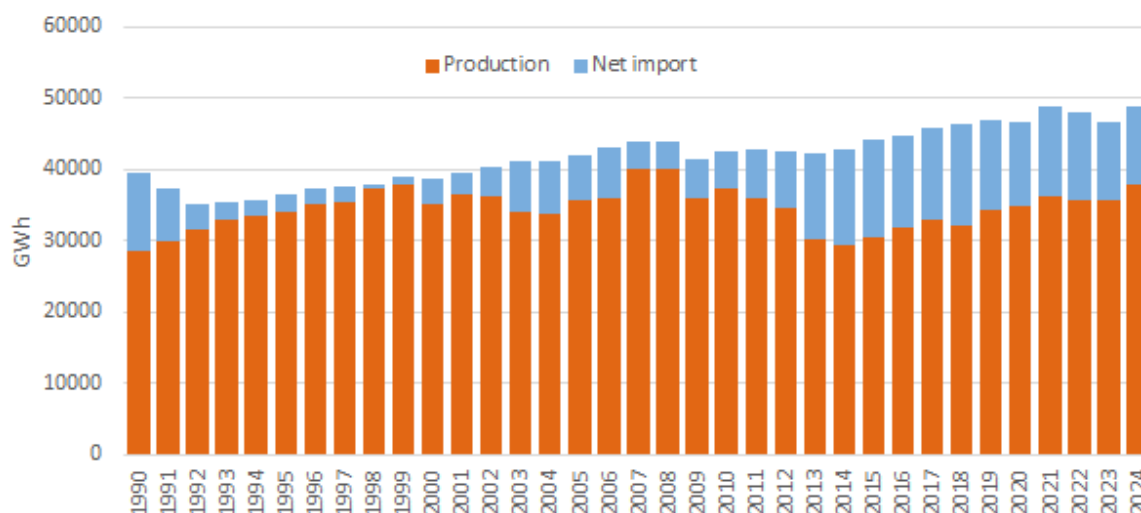
Figure 3.2.5.2 Domestic Electricity Production and Net Import (1990-2024)
