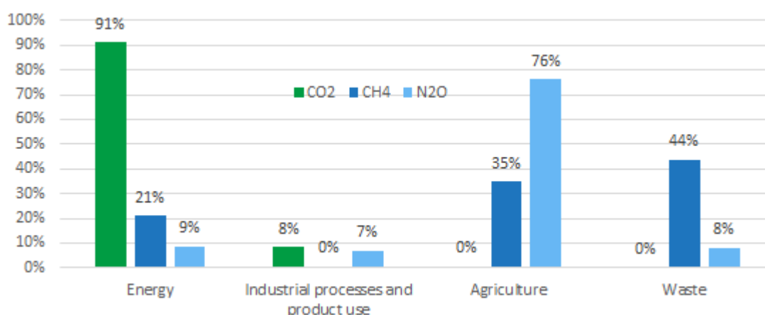
Figure 3.1.2 Sectoral contributions to the total emissions of the main GHG gases (2024)
