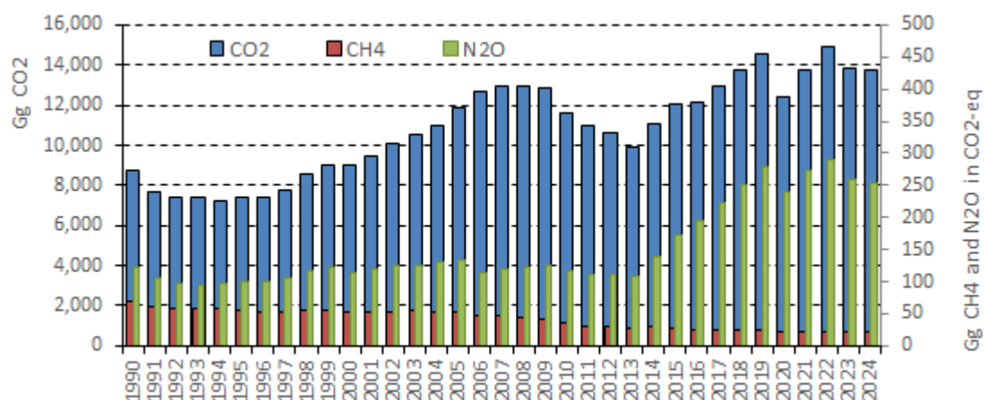
Figure 3.2.7.5 Trends of CO 2 , CH 4 and N 2 O emissions in the Transport Sector (1990-2024)
