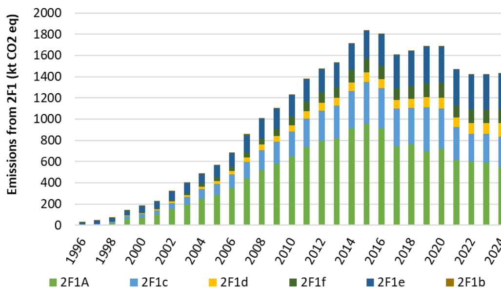
Figure 4.8.2 Emission from 2.F.1 by subcategories
