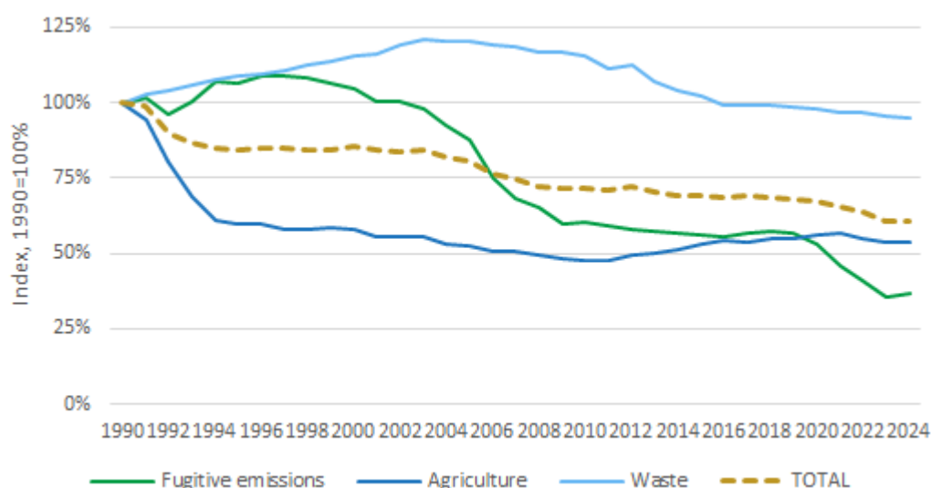
Figure 2.11 Trend of CH 4 emissions from some selected important sources
