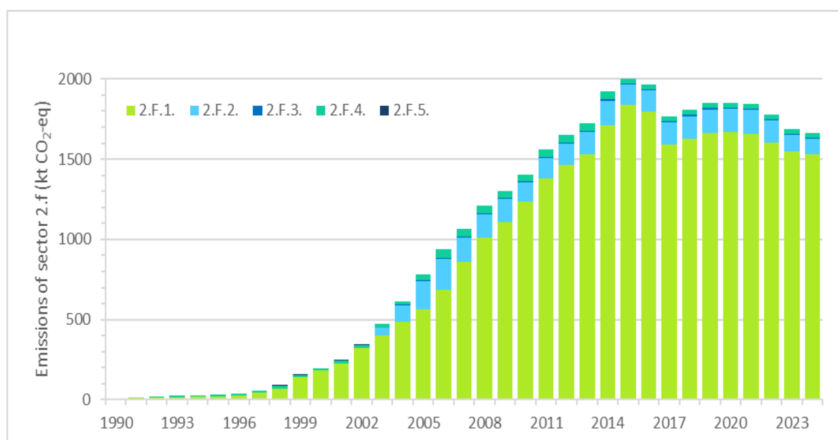
Figure 4.8.1 Trend of emission from 2.F.1 between 1990 and 2023 (kt CO 2 -eq)
