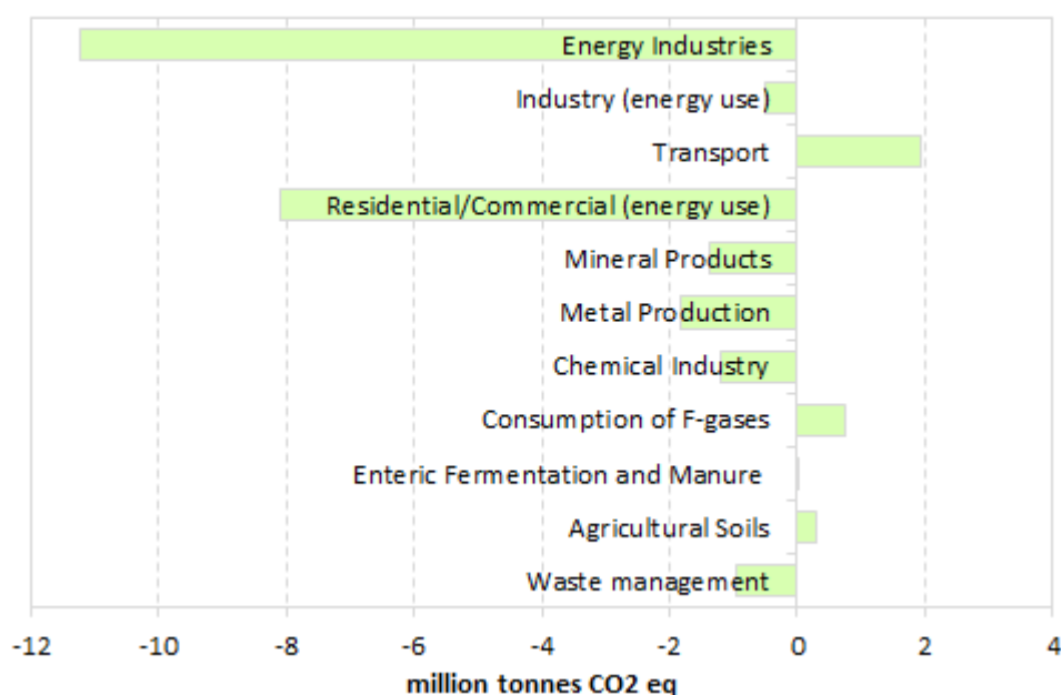
Figure 2.5 Changes in emissions between 2005 and 2024, million tonnes CO 2 -eq
