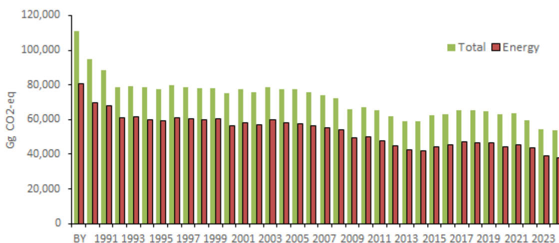
Figure 3.1.2 GHG emissions of the Energy sector compared to total (BY-2024)
