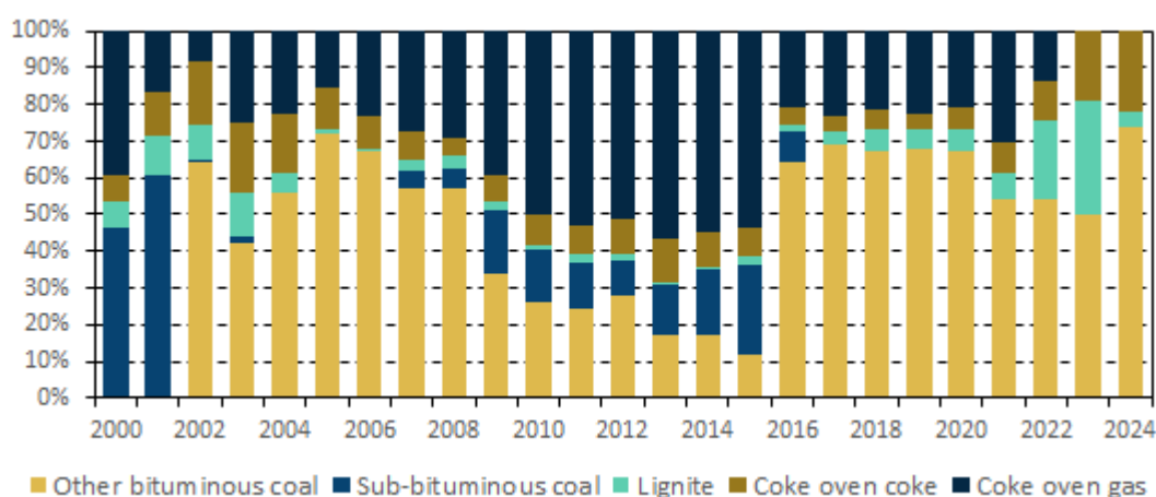
Figure 3.2.6.4 Share of different solid fuels used by manufacturing industries (2000-2024)
