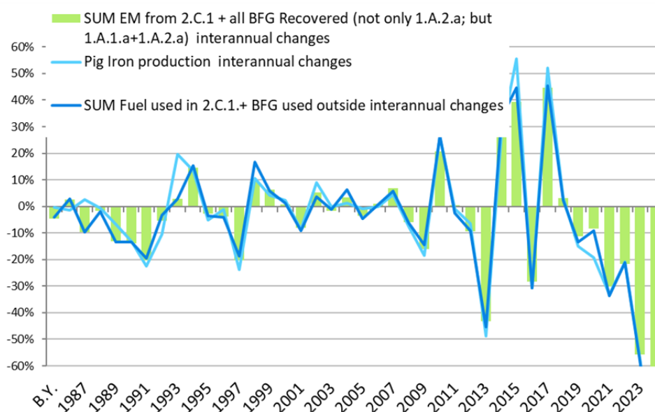
Figure 4.6.2 Comparison of trends of pig iron production, fuel use and the emissions allocated in different sectors in HU GHG inventory
